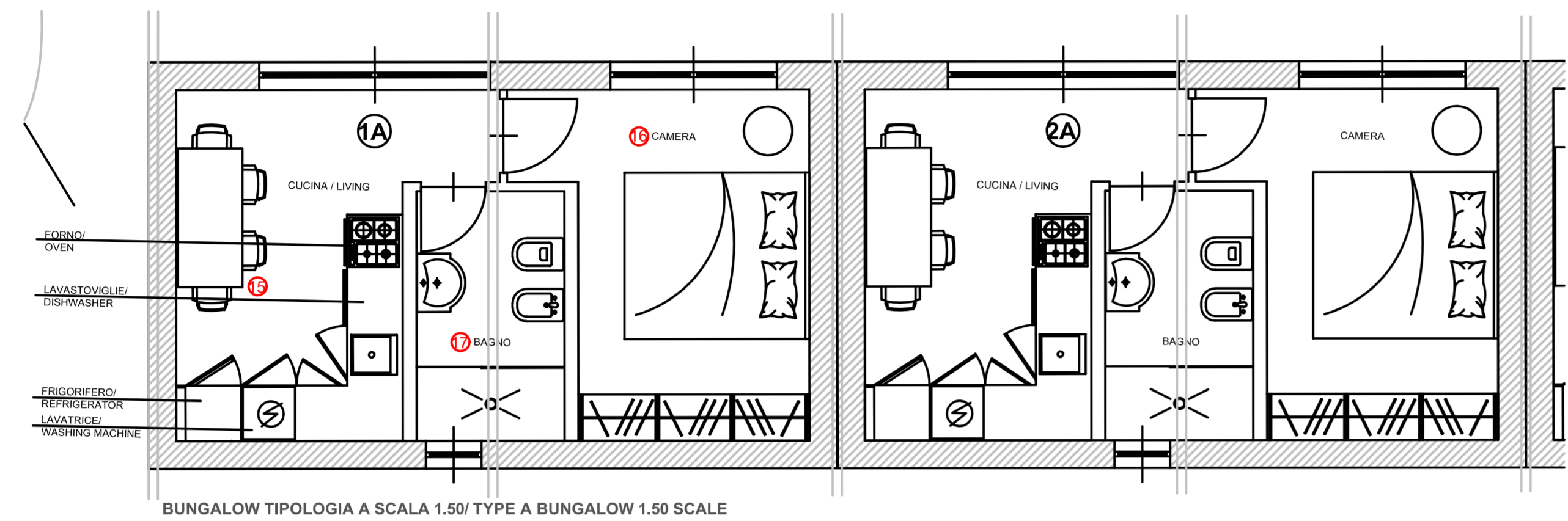
BUNGALOW TIPOLOGIA A SCALA 1:50 / TYPE A BUNGALOW 1:50 SCALE
