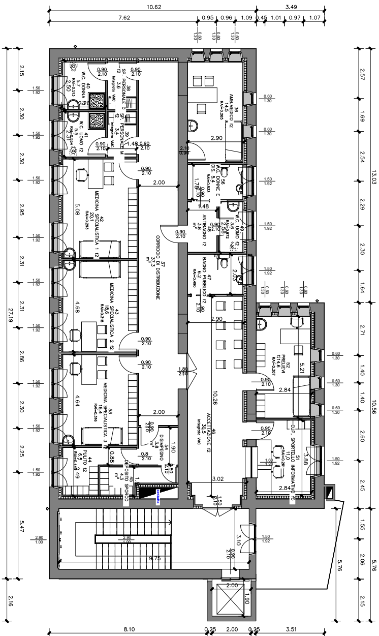
PIANO SECONDO SDP Sc 1 : 100
