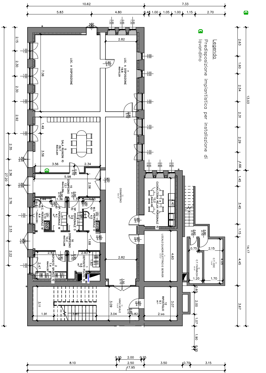
PIANO SEMINTERATO-TERRA SDP Sc 1 : 100
