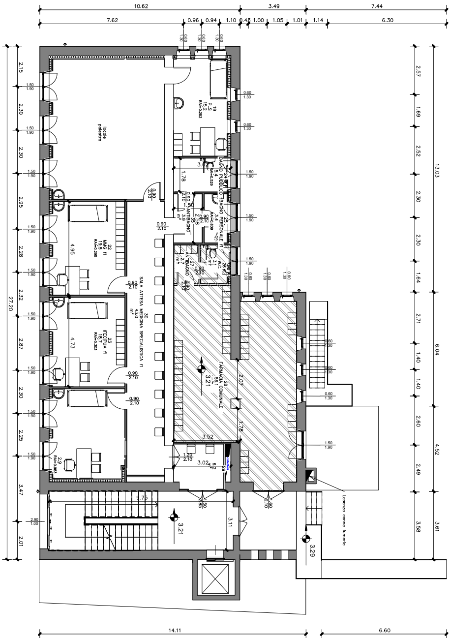
PIANO PRIMO SDP Sc 1 : 100
